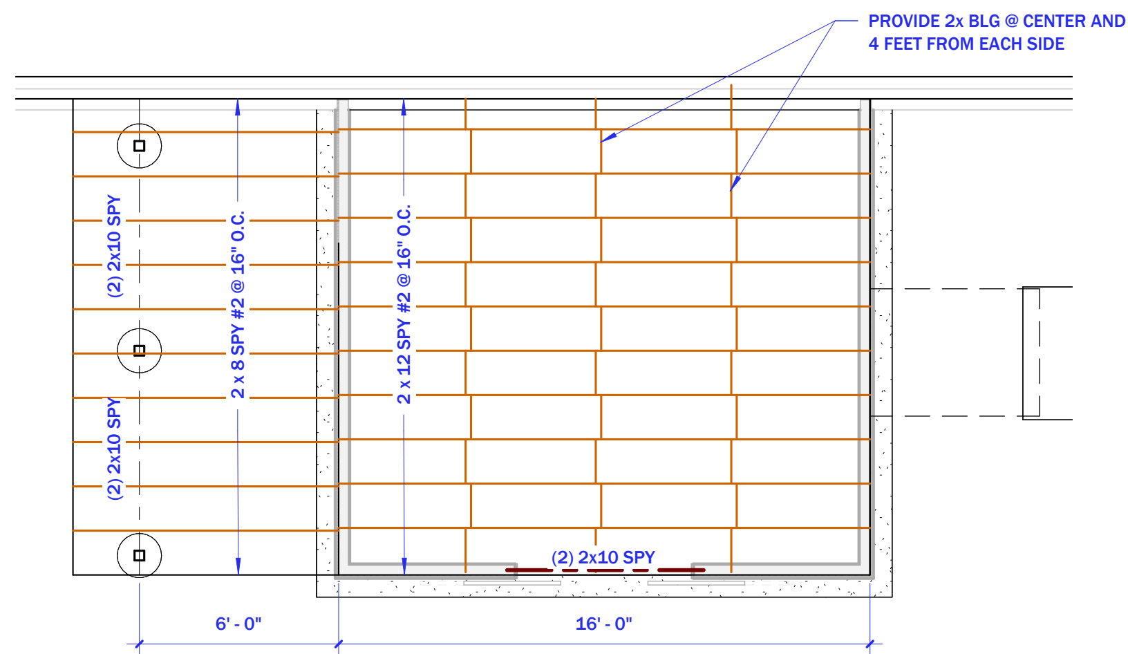
12 FRAMING PLAN 1/4" = 1'-0"
