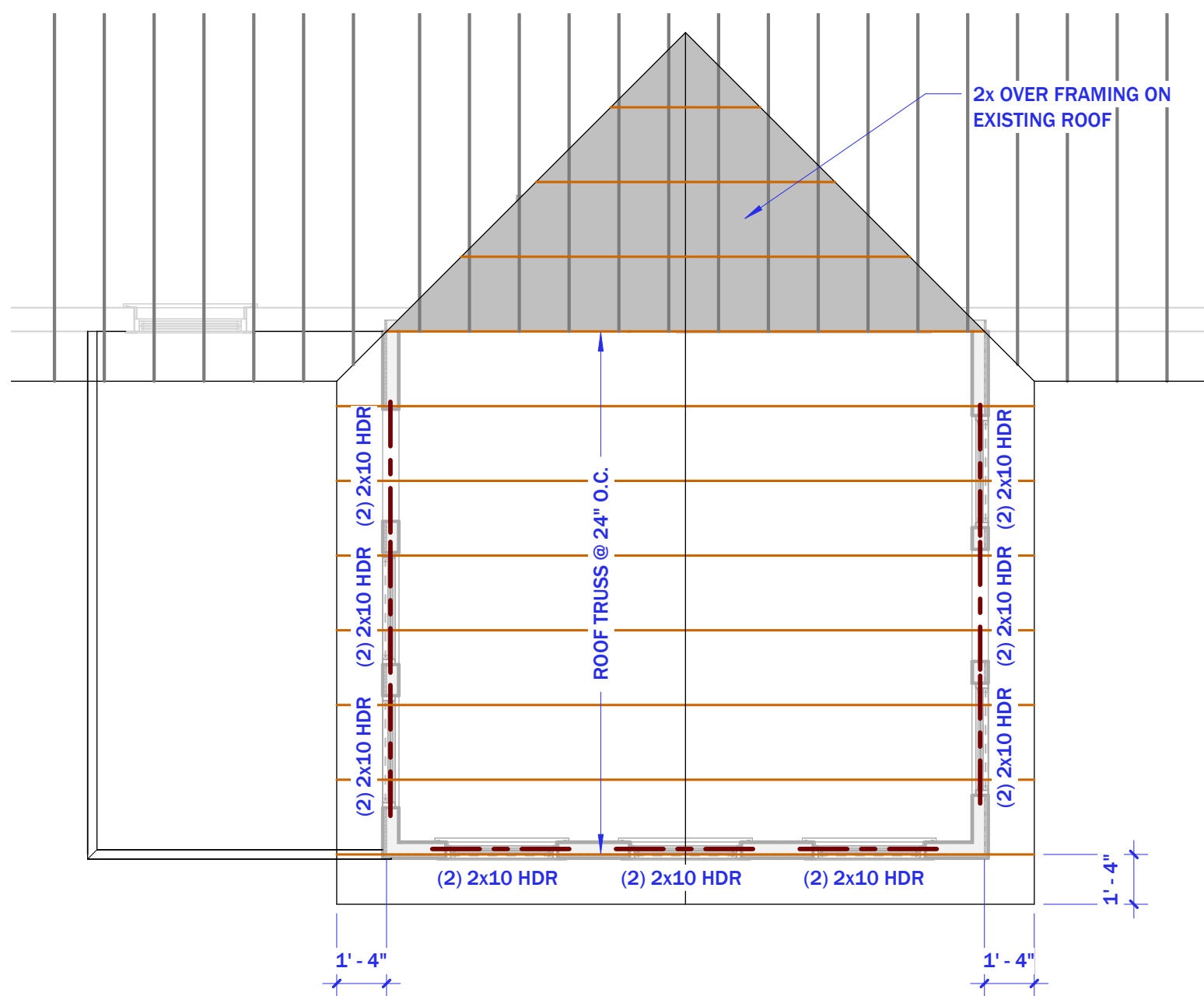
13 ROOF FRAMING PLAN 1/4" = 1'-0"
