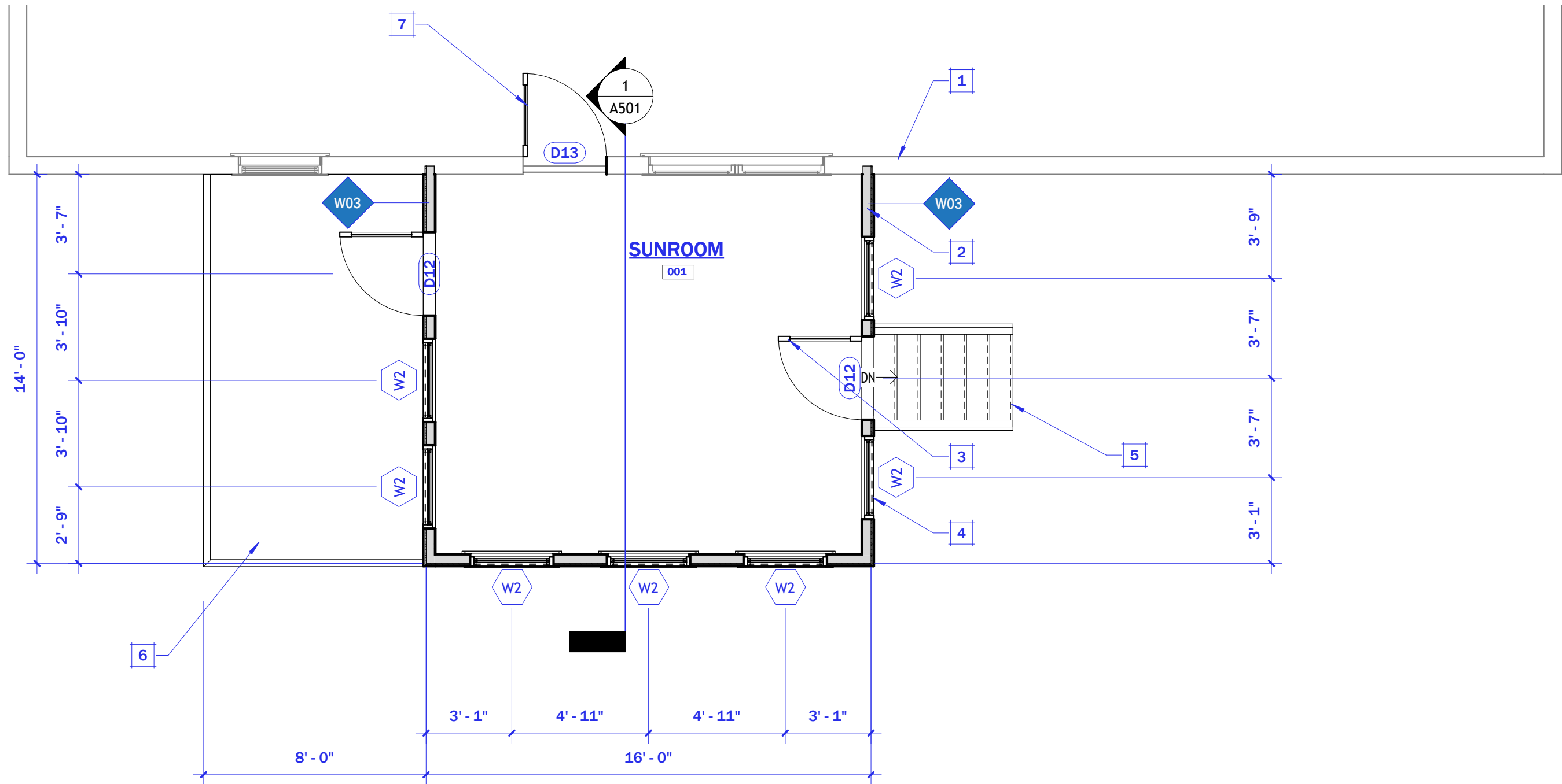
1 MAIN LEVEL FLOOR PLAN 1/4" = 1'-0"
