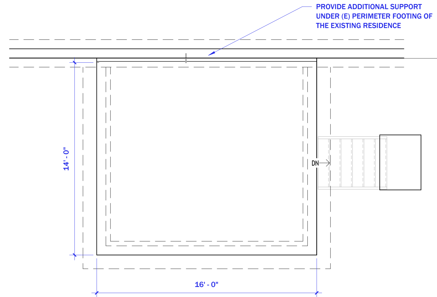
11 FOUNDATION PLAN 1/4" = 1'-0"
