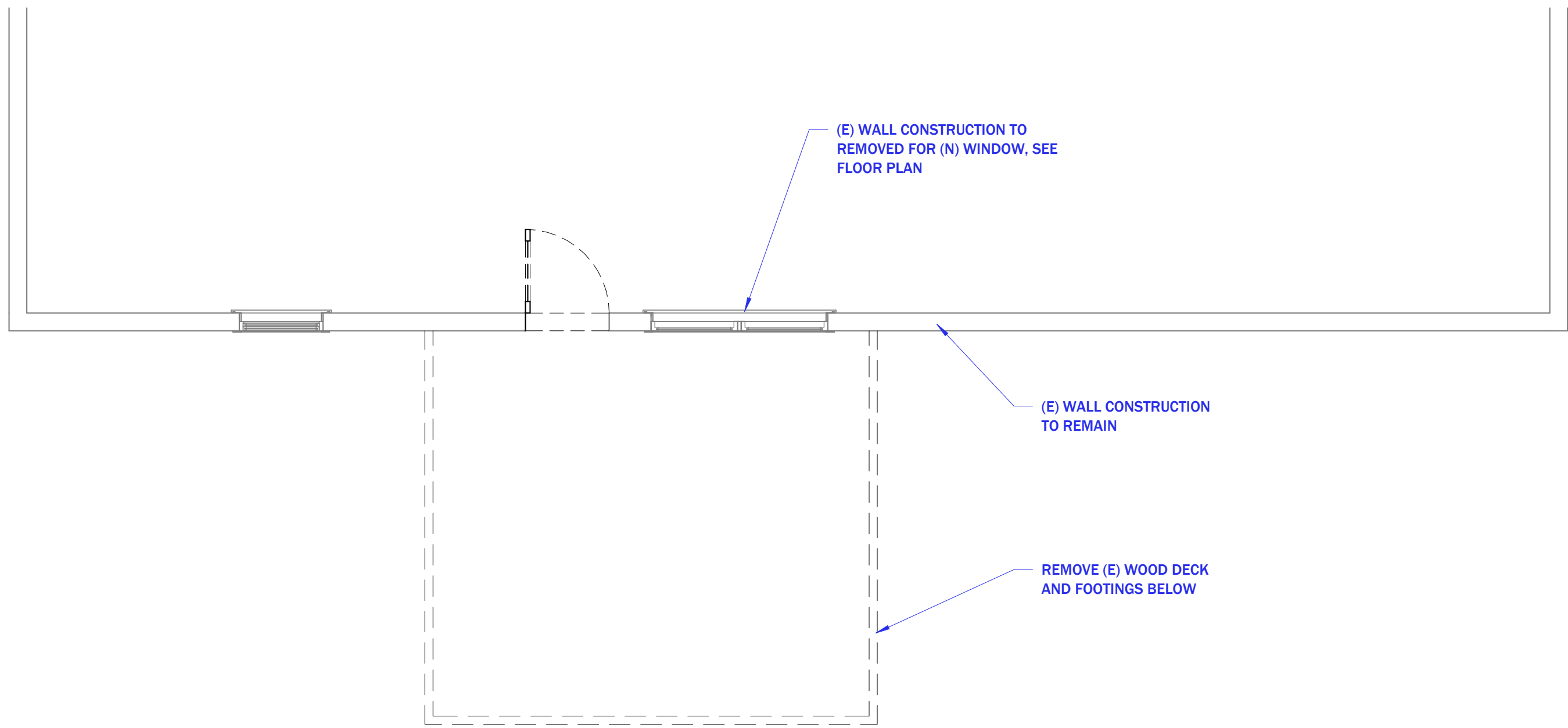
2 DEMO PLAN 1/4" = 1'-0"
