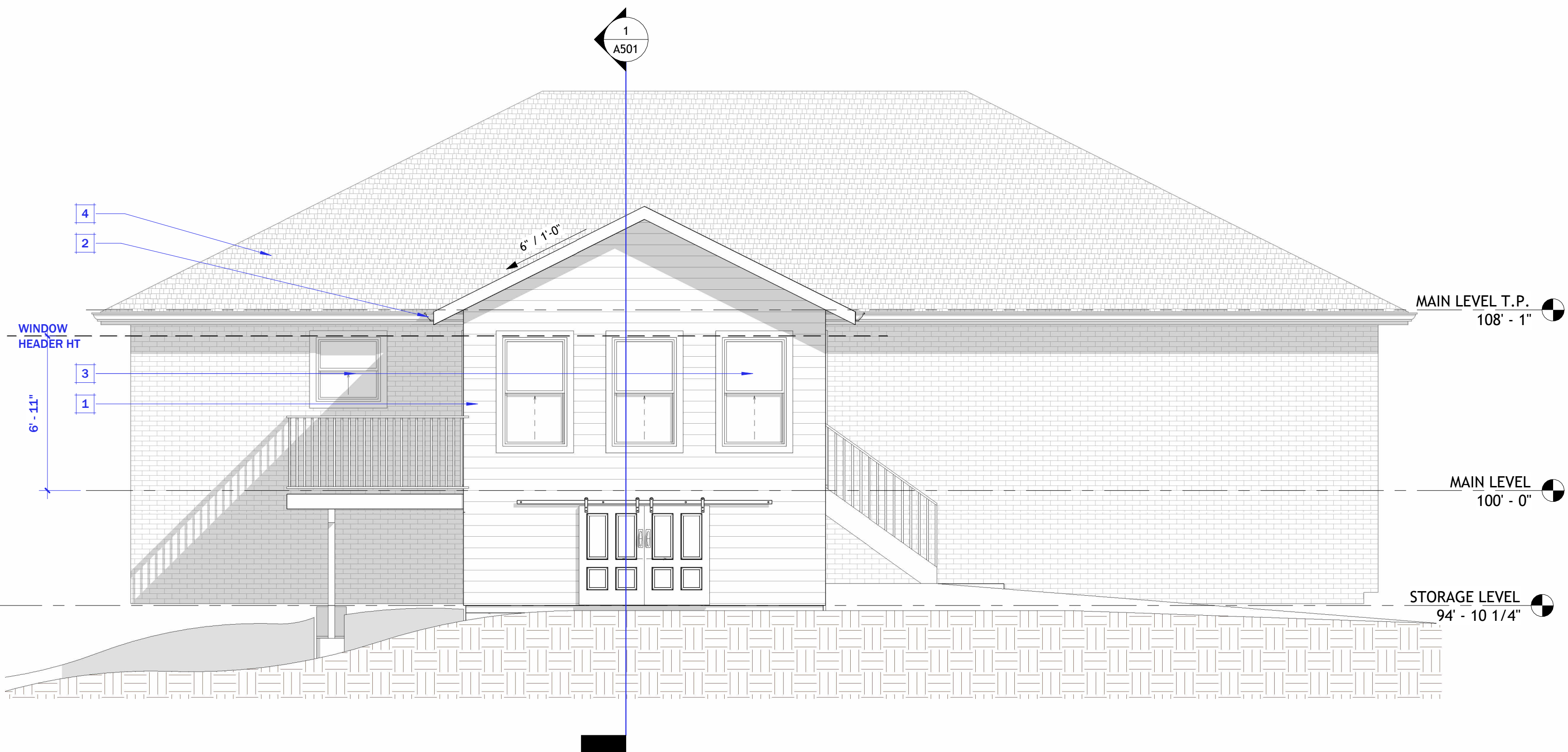
2 REAR EXTERIOR ELEVATION 1/4" = 1'-0"
