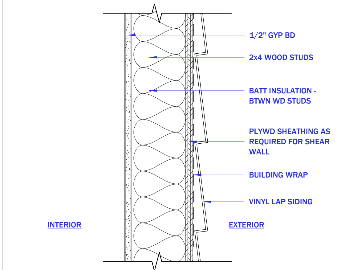
3 WALL TYPE - W03 3" = 1'-0"
