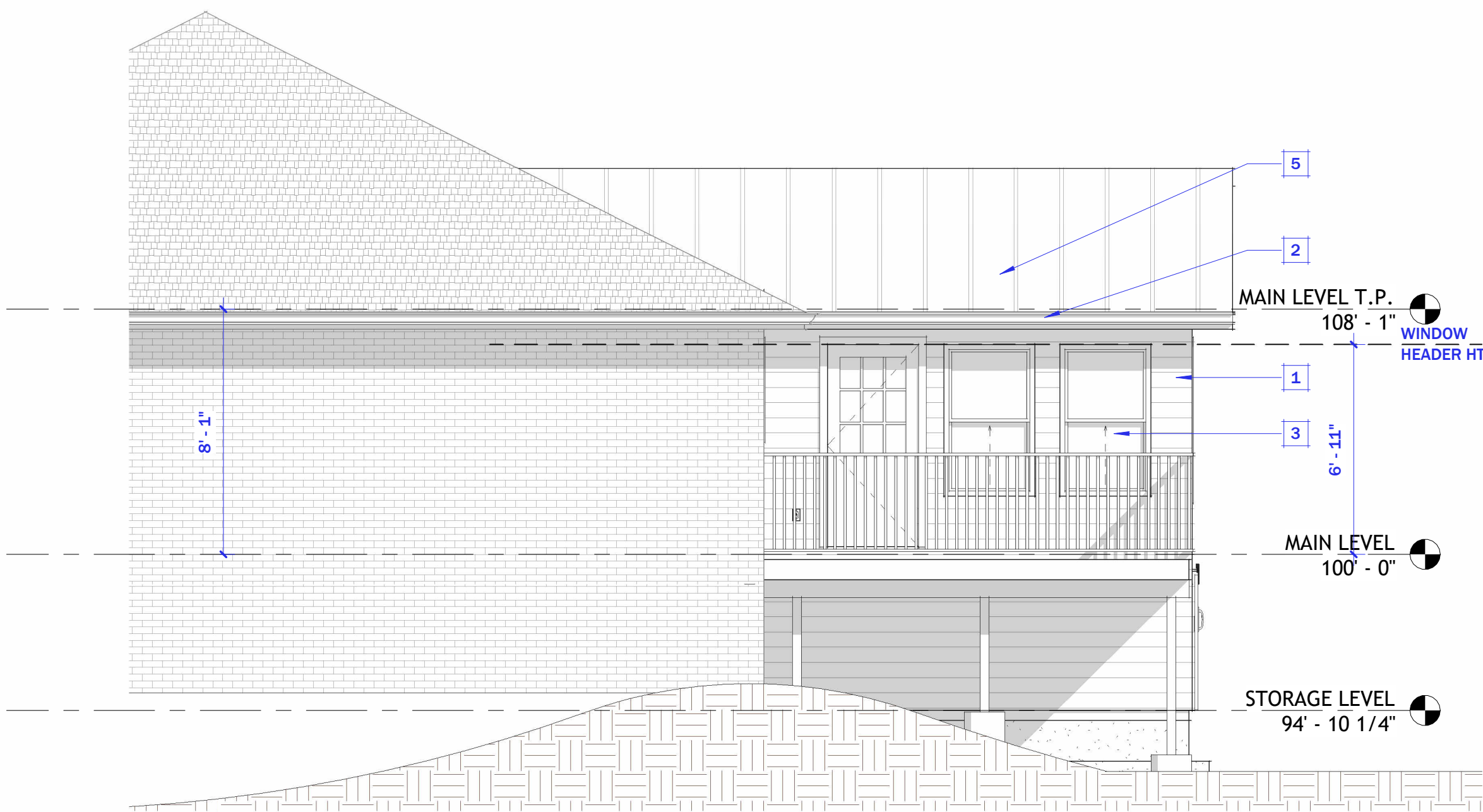
1 NORTH EXTERIOR ELEVATION 1/4" = 1'-0"
