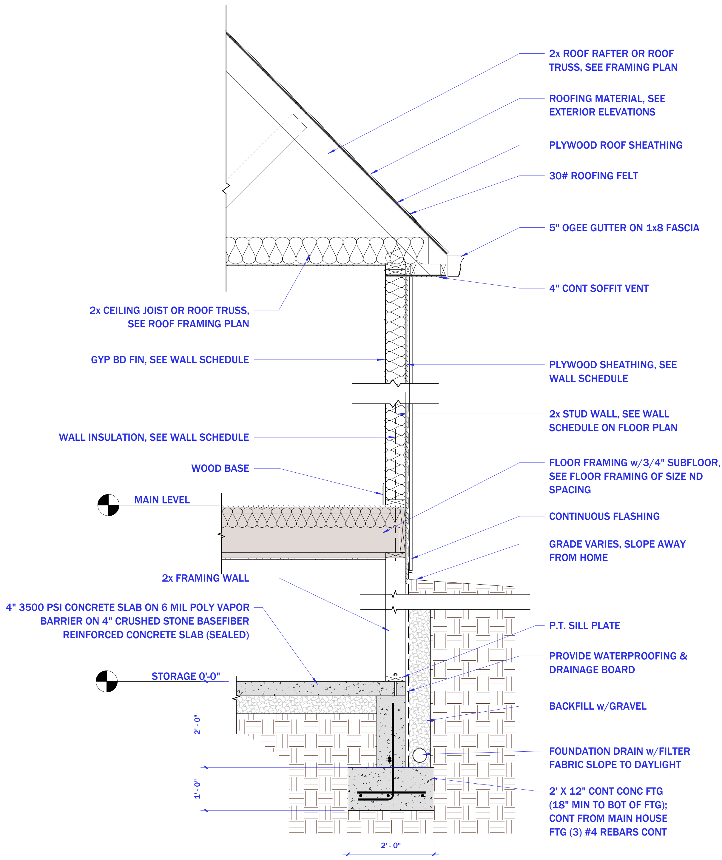
33 TYPICAL WALL SECTION FRAMED WALL 3/4" = 1'-0"
