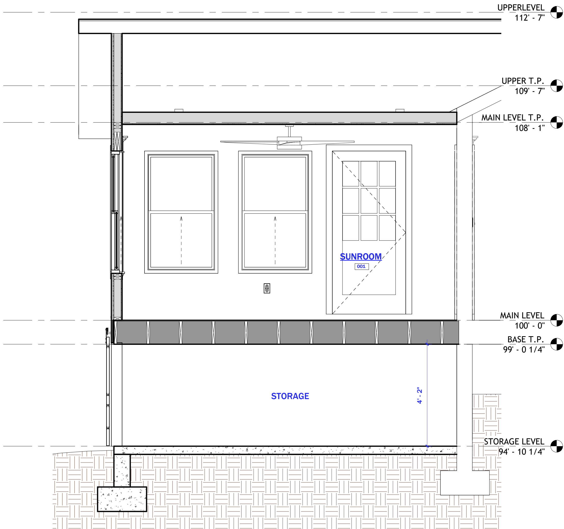
1 Section 2 1/2" = 1'-0"
